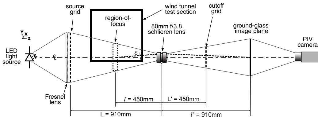
Fig. 2 Schematic of the focusing schlieren optical system.
