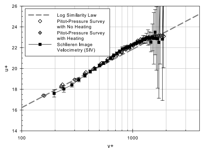
Fig. 13 Mean subsonic boundary-layer velocity-profile data measured with pitot-pressure survey and SIV, processed with the MATLAB program. The boundary-layer edge is at y+ \approx 1430 . The error bars represent 1 standard deviation from the mean on the SIV results.
