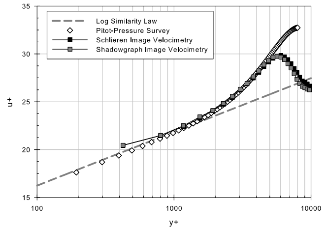
Fig. 12 Mach 3 mean boundary-layer velocity-profile data measured with pitot-pressure survey and schlieren PIV techniques, plotted in wall-wake coordinates. The boundary-layer edge is at y+ \approx 7900 .
