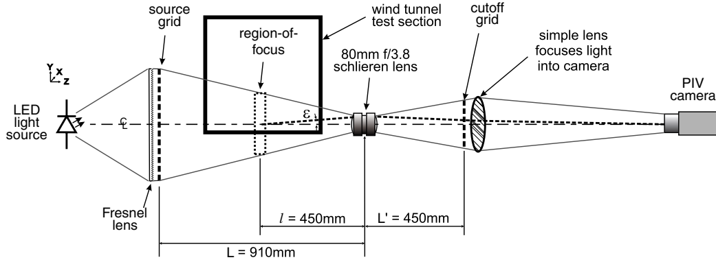
Fig. 3 Schematic of the final focusing schlieren optical system with a simple lens used to focus the schlieren beam into the camera.
