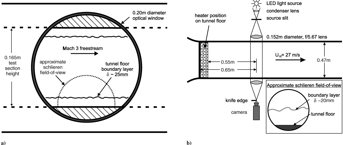
Fig. 1 Schematics of a) supersonic wind-tunnel test section and the approximate area being imaged and b) top view of the subsonic wind-tunnel experimental setup, including the lens-type schlieren system used for both subsonic and supersonic schlieren and shadowgraph imaging.
