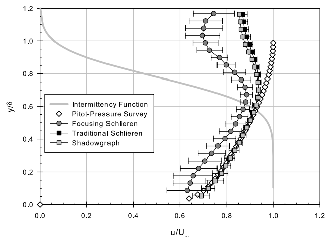
Fig. 11 Mach 3 mean boundary-layer velocity-profile data measured with pitot-pressure survey and SIV techniques, processed with the MATLAB program. The error bars represent the standard deviation of the average and are approximately the same for the schlieren and shadowgraph measurements.
