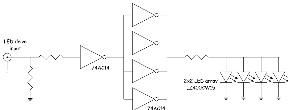
Fig. 7 Circuit diagram for the 2 \times 2 LED array.
