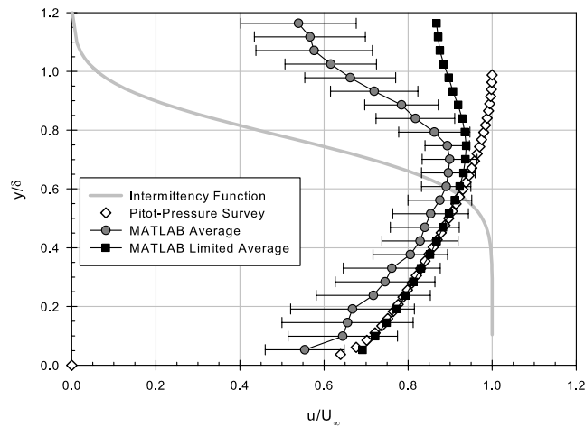
Fig. 10 Mach 3 mean boundary-layer velocity-profile data measured with pitot-pressure survey and SIV, also showing turbulent boundary-layer intermittency function. The error bars represent the standard deviation of the average and are approximately the same for the schlieren and shadowgraph measurements.
