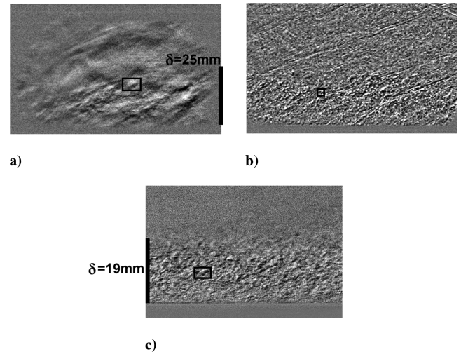
Fig. 5 Images of tunnel-floor boundary layers: a) focusing schlieren image of M = 3 boundary layer, b) focused shadowgraph of M = 3 boundary layer, and c) parallel-light schlieren image of thermally seeded subsonic boundary layer. The scale in each image shows the height of the boundary-layer edge, measured from the tunnel floor, which is at the base of the vertical scale mark. The interrogation window for each image series is also shown in each image as a rectangular box. The interrogation-window sizes are selected to fully encompass a typical turbulent structure.
